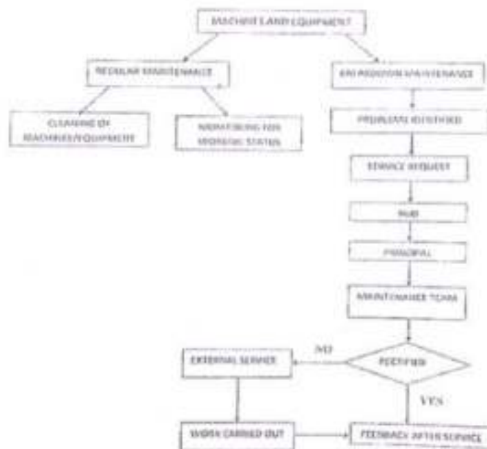
FLOW CHART FOR MACHINES AND EQUIPMENT MAINTENANCE
